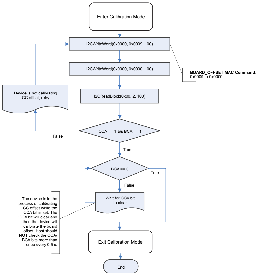
Figure 3-2. Board Offset Flow
