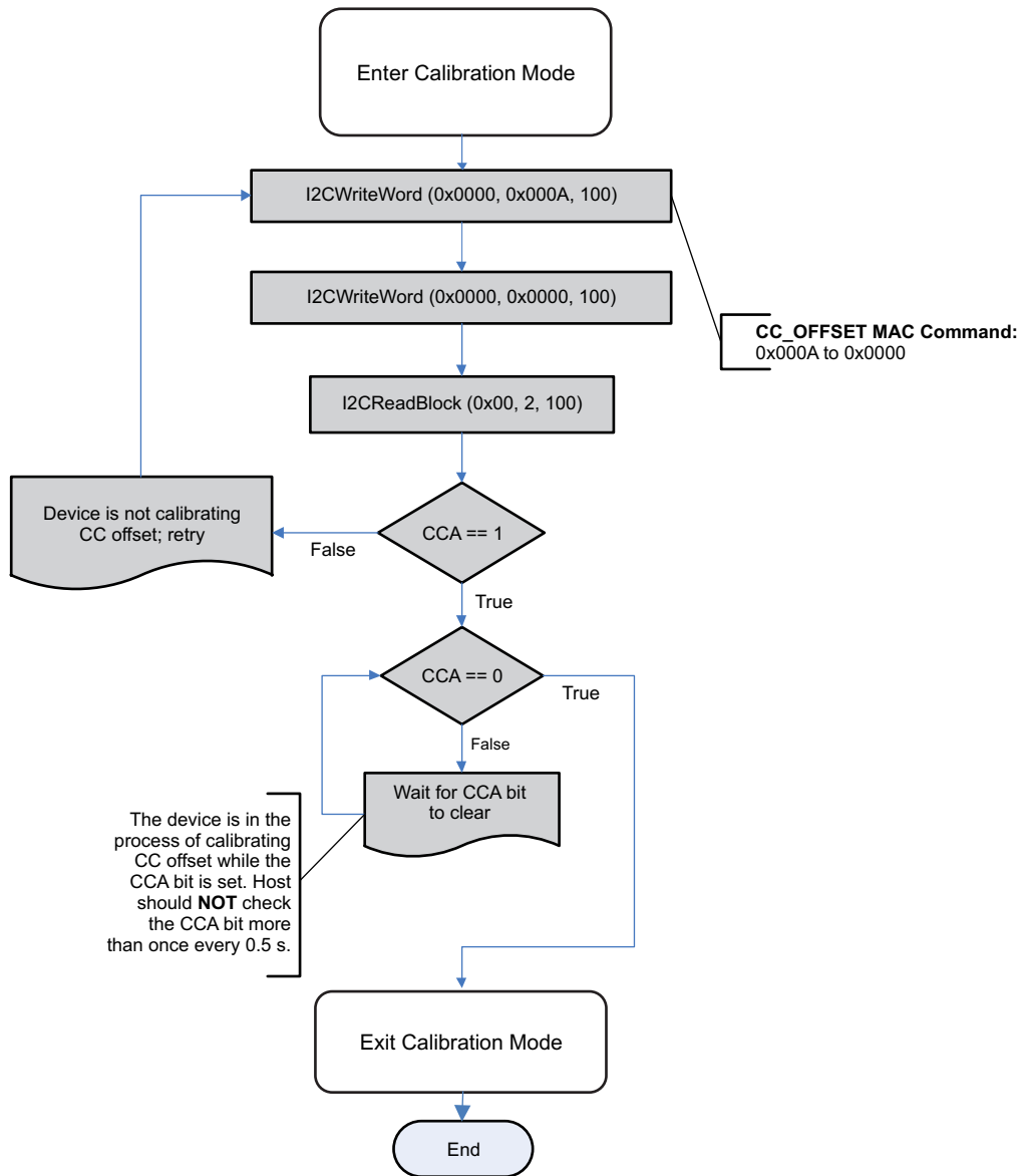
Figure 3-1. CC Offset Flow
