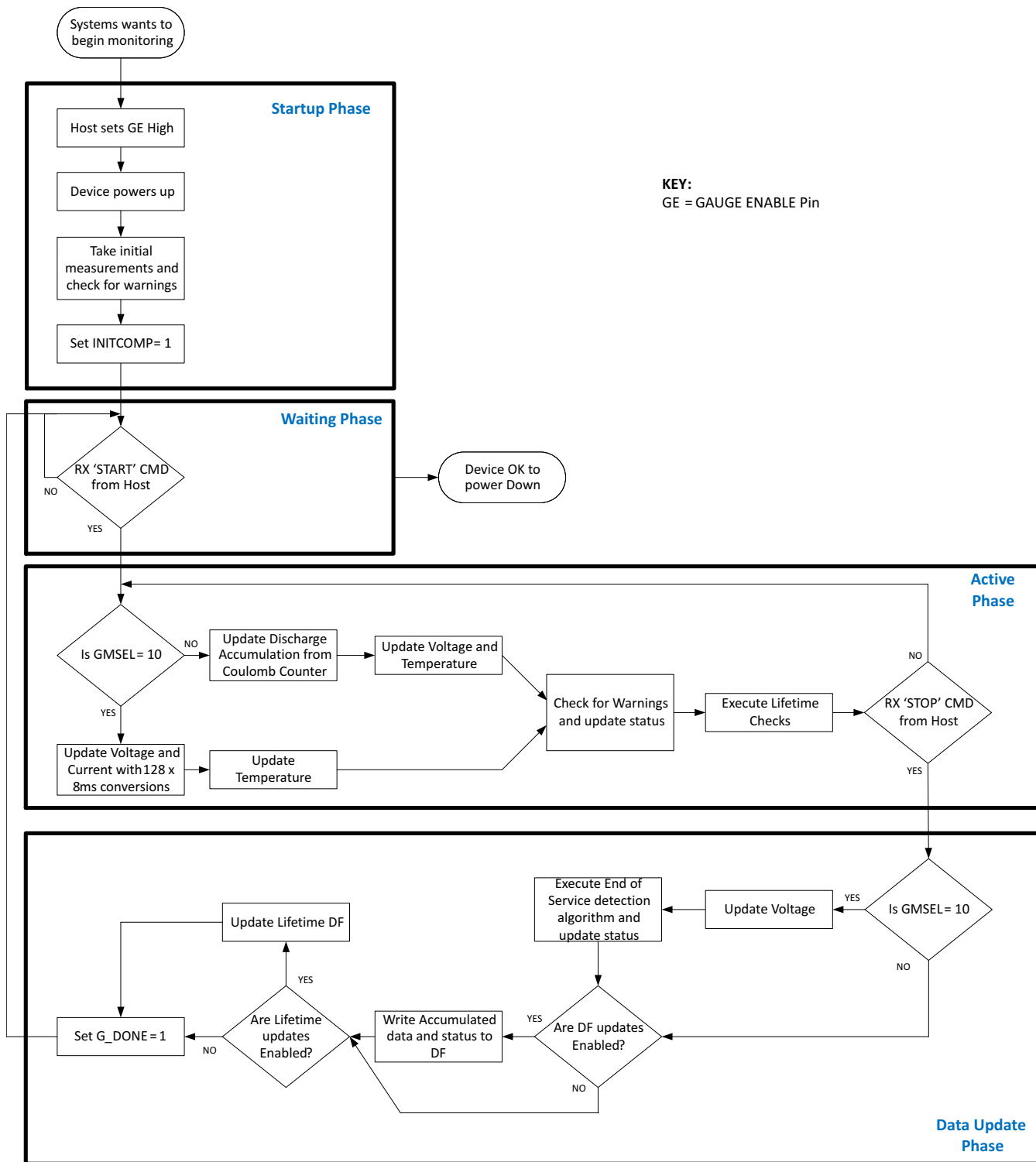
Figure 11. Operational Flow
